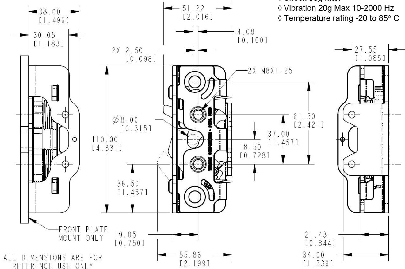
Base Latch Shown Without Actuators
